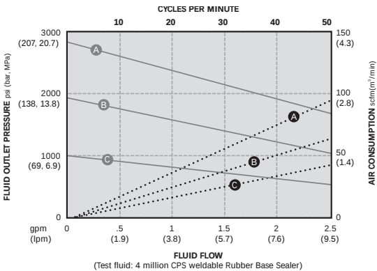
Performance Chart for 31:1 Bulldog Check-Mate 800 Pump
