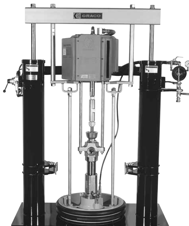
C59702 Dura-Flo Ram Pump
